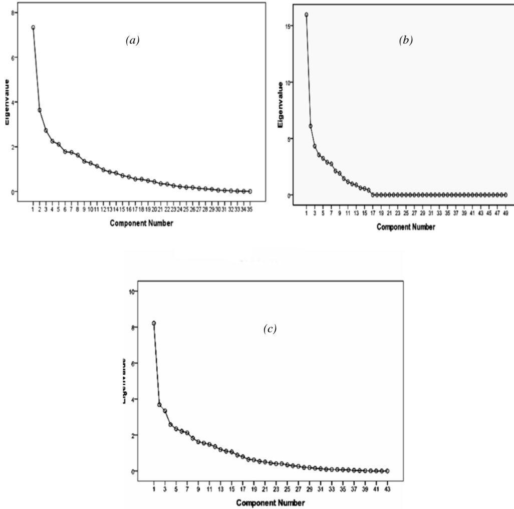
Web Fig. 1 Scree Plot (a) 6-13 years format (b) Adolescent's format (c) Parents' format. The point at which the plot sharply dips is the maximum number of factors recommended. Our analysis suggests reduction of the number of domains for Hindi CFQ-R to 5, 7 and 2 for 6-13, Adolescent's and Parents' formats, respectively.
