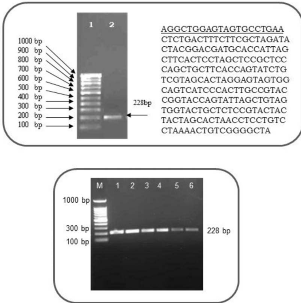
Web Fig. 1 Top panel: Lane 1: DNA Ladder 100bp; Lane 2: purified PCR product (228 bp). Bottom panel: sof gene as a specific genetic marker for detection of Streptococcus pyogenes .
