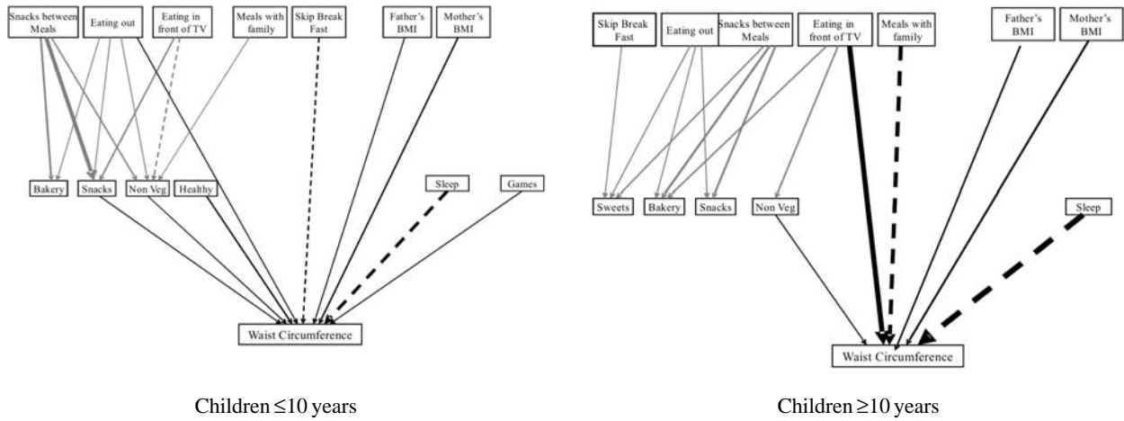
WEB FIG.1 Path diagram depicting possible causal mechanism of various factors to waist circumference. Value of path coefficients are represented as the thickness of the line where a standard regression coefficient of 0.1 is equivalent to 0.5 points in the diagram. Solid Line - positive relationship with WC; Dashed Line - negative relationship with WC.
